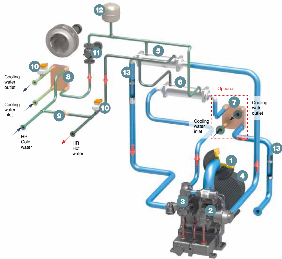
CSG – Water-cooled version with heat recovery
